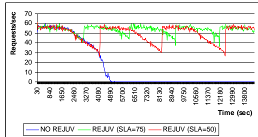
Figure 4: Applying Rejuvenation to TPC-W.
