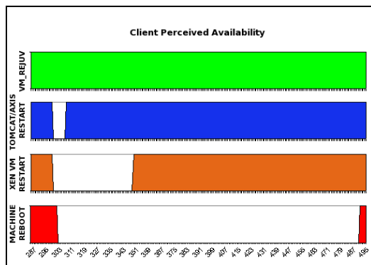
Figure 5: Client Perceived Availability for Different Restart Mechanisms (Tomcat/Axis).
