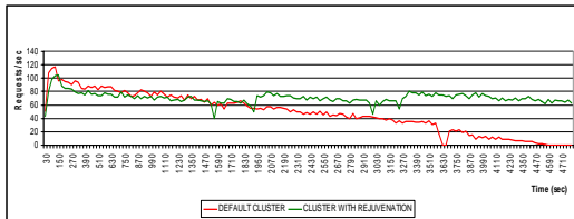
Figure 8: Comparing the cluster throughput, with and without rejuvenation and no automatic restart (Tomcat/Axis)
