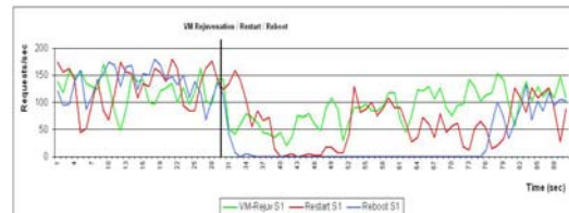
Figure 10: The impact of a “clean” restart when compared with a “blind” restart and a “blind” reboot (Tomcat/Axis).
