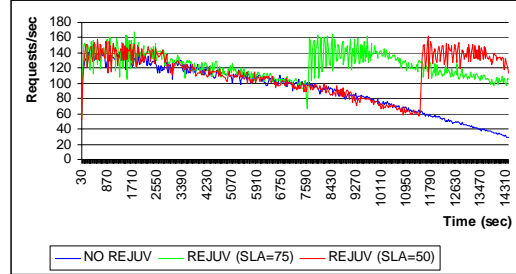
Figure 3: Applying Rejuvenation to Tomcat/Axis.
