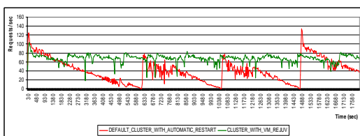
Figure 9: Comparing the cluster throughput, with and without rejuvenation, but automatic restart (Tomcat/Axis).
