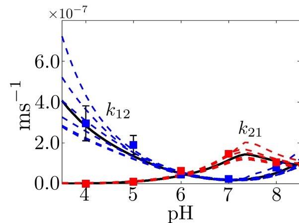
(b) Transition rates
