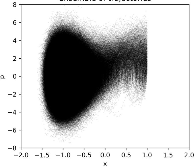
Ensemble of trajectories
