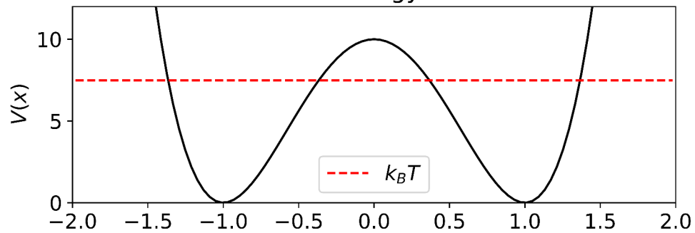
Potential energy function
