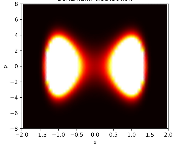
Boltzmann distribution
