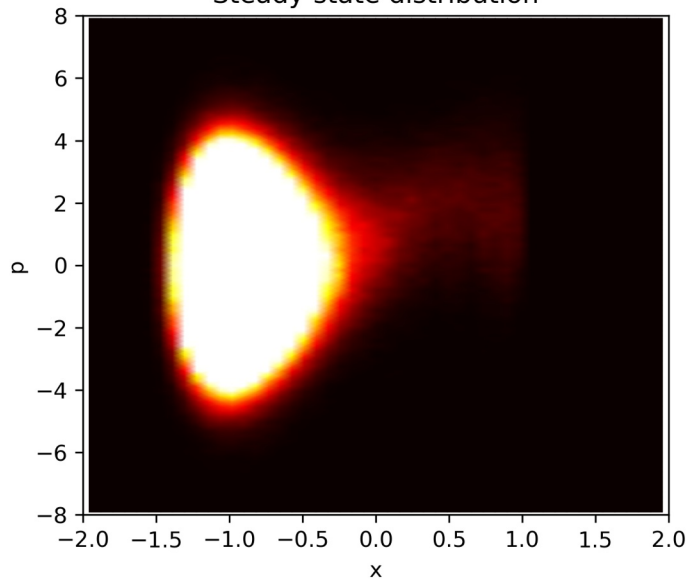
Steady-state distribution
