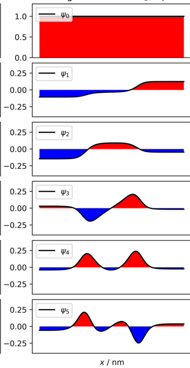
Eigenfunctions of Q, \mathcal{K}_\tau
