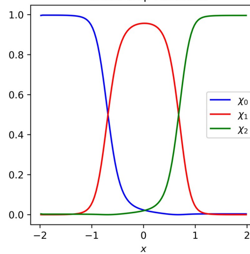
Membership functions
