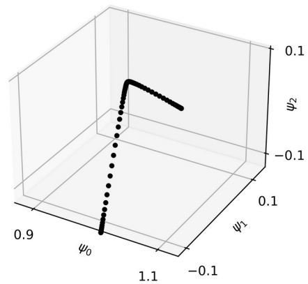
2-simplex \psi_0, \psi_1, \psi_2
