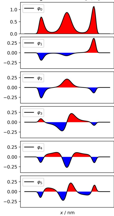
Eigenfunctions of Q^*, P_\tau
