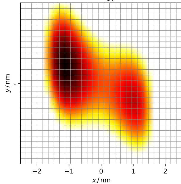
Potential energy function
